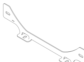
BOTTOM BRACKET Part No. 130199 x1
